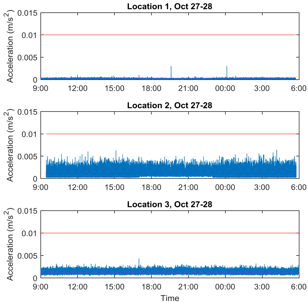
Figure 1: RMS particle accelerations at Location 1, 2 and 3 on October 27-28, 2017. The magenta dash line represents the mean baseline RMS particle acceleration calculated from October 5 to 16 at each location. The red line shows the 0.01 m/s 2 threshold of the RMS particle acceleration.
